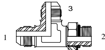
(1)(3) Male JIC (2) Male BSPP Adjustable Run Tee C/W Retaining Ring & O-Ring
