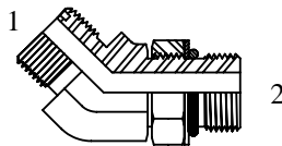
(1) Male 45 BSPP (2) Male BSPP Adjustable C/W Retaining Ring & O-Ring
