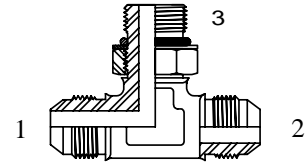
(1)(2) Male JIC (3) Male BSPP Adjustable Branch Tee C/W Retaining Ring & O-Ring
