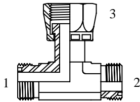
(1) (2) Male BSPP (3) Female BSPP Swivel Branch Tee
