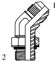
(1) Male 45 JIC (2) Male BSPP Adjustable C/W Retaining Ring & O-Ring
