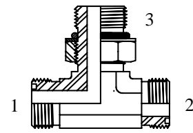
(1) (2) Male BSPP (3) Male BSPP Branch Tee C/W Retaining Ring & O-Ring
