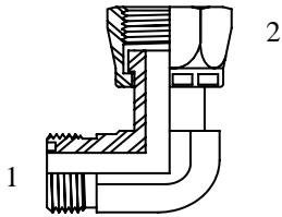
(1) Male 90 BSPP (2) Female BSPP Swivel
