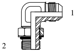
(1) Male 90 JIC (2) Male BSPP Adjustable C/W Retaining Ring & O-Ring
