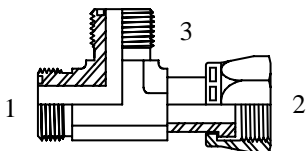
(1) (3) Male BSPP (2) Female Swivel Run Tee
