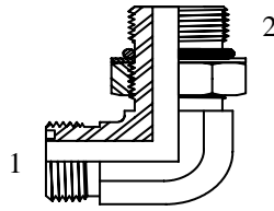
(1) Male 90 BSPP (2) Male BSPP Adjustable C/W Retaining Ring & O-Ring
