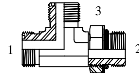
(1) (3) Male BSPP (2) Male BSPP Run Tee C/W Retaining Ring & O-Ring
