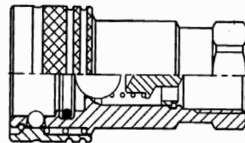
FEMALE BODY
