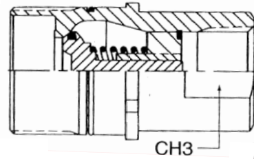
BRASS PLUG
