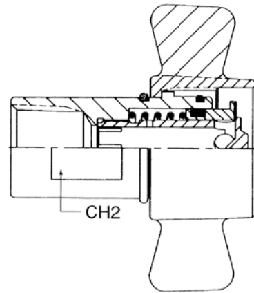
BRASS COUPLER
