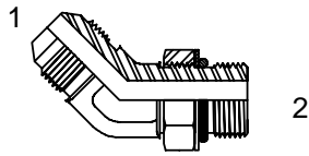
(1) 37° MALE (2) MALE "O" RING
