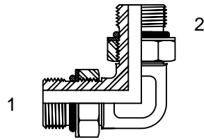
(1-2) ADJUSTABLE "O" RING
