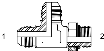
(1-3) 37° MALE (2) MALE "O" RING
