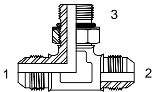
(1-2) 37° MALE (3) MALE "O" RING
