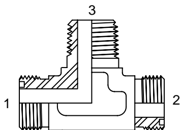
(1) (2) MALE ORFS (3) MALE PIPE
