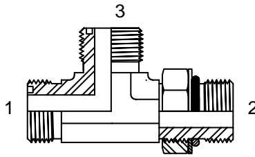
(1)(3) MALE ORFS (2) ADJ. O-RING
