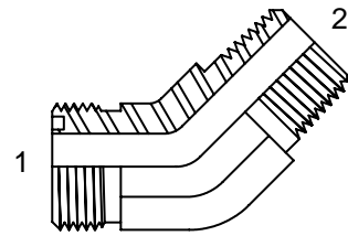
(1) MALE ORFS (2) MALE PIPE
