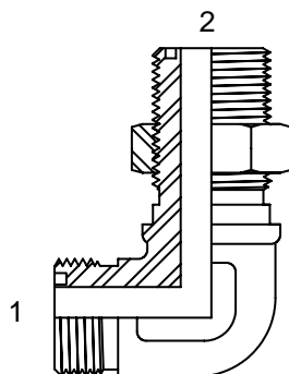
(1) MALE ORFS (2) ORFS BULKHEAD
