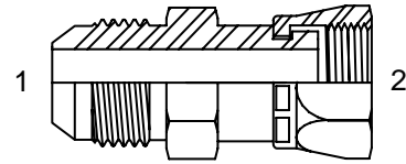
(1) JIC MALE TUBE (2) ORFS FEMALE SWIVEL
