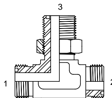
(1) (2) MALE ORFS (3) ORFS BULKHEAD
