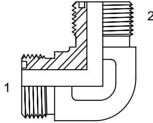
(1) MALE ORFS (2) MALE PIPE
