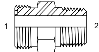
(1) MALE ORFS (2) MALE PIPE
