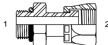
(1) MALE O-RING (2) ORFS FEMALE SWIVEL
