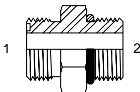
(1) MALE ORFS (2) MALE O-RING
