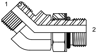
(1) MALE ORFS (2) ADJ. O-RING
