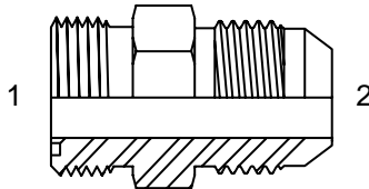
(1) MALE ORFS (2) JIC MALE TUBE
