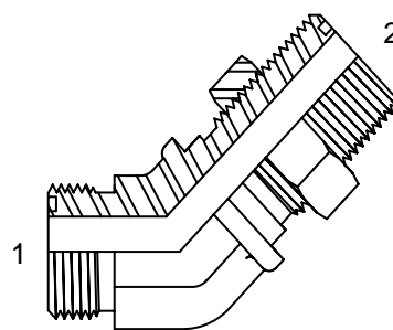
(1) MALE ORFS (2) ORFS BULKHEAD
