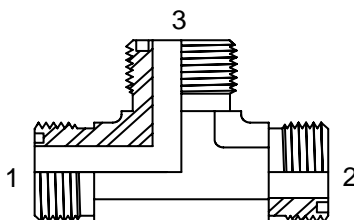
(1)(2)(3) MALE ORFS
