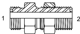
(1) MALE ORFS (2) ORFS BULKHEAD
