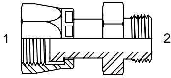
(1) ORFS FEMALE SWIVEL (2) MALE ORFS
