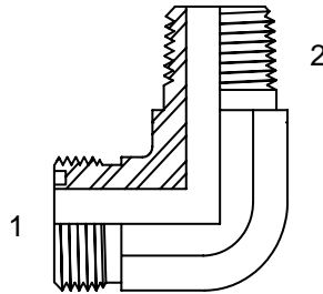
(1) MALE ORFS (2) MALE PIPE
