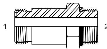
(1) MALE ORFS LONG (2) MALE O-RING
