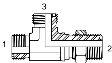
(1) (3) MALE ORFS (2) ORFS BULKHEAD
